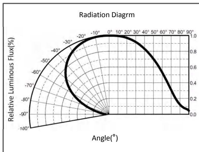
f) Beam Angle Characteristics 光束角 ( I_F = 350\text{ mA} , T_J = 25^\circ\text{C} )
