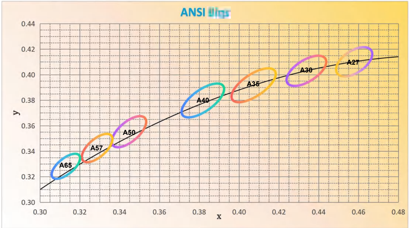
f) Chromaticity Region & Coordinates 色度区域与坐标 ( I_f = 350 \text{ mA} , T_j = 25^\circ \text{C} )
